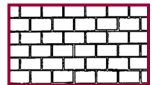
LARGE STRETCHER BOND Brick size: 240mm x 115mm
